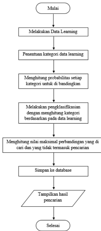
Gambar. 1. Alur Metode Naïve Bayes
